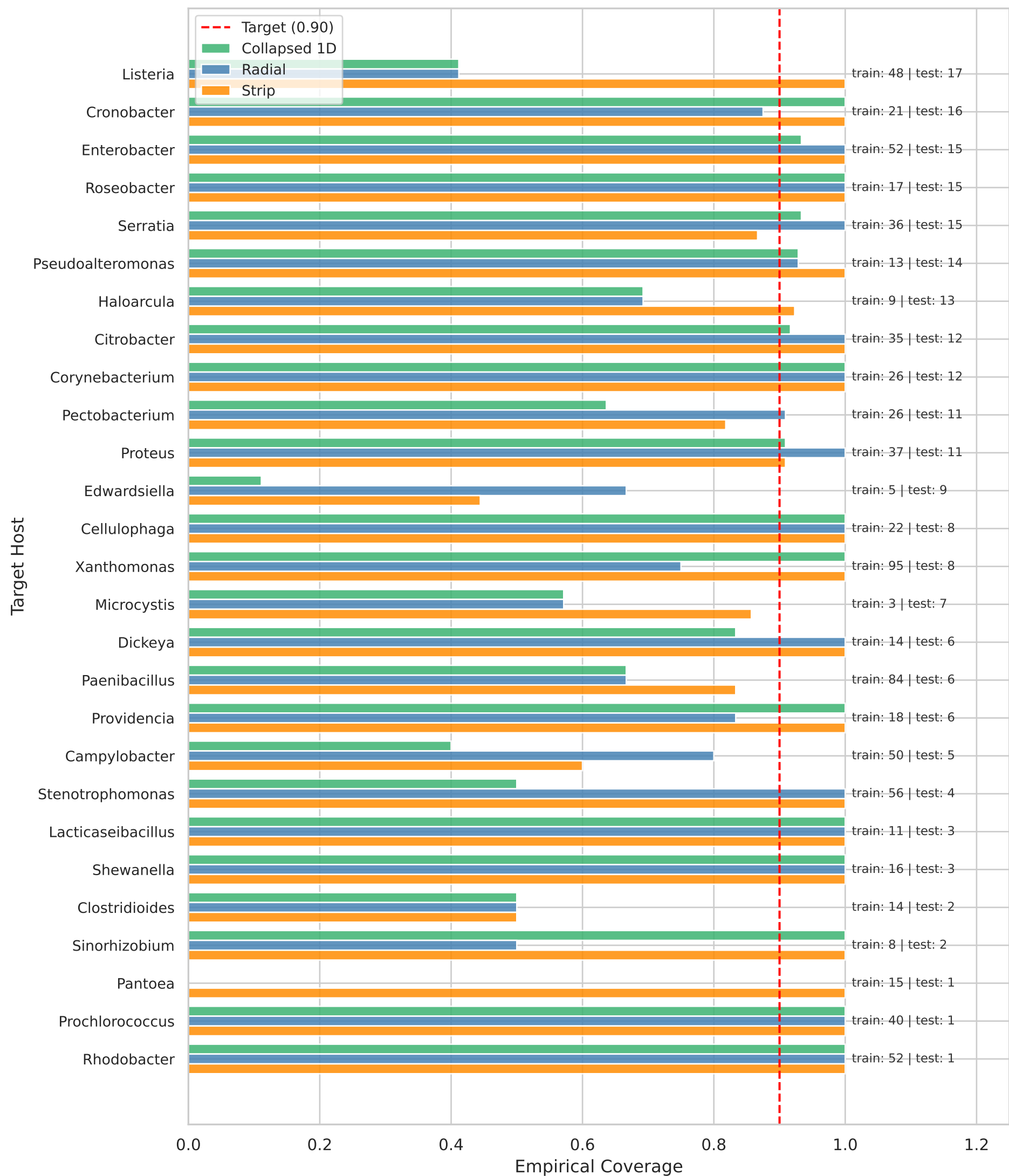
Class Conditional Coverage Breakdown Per Host (All Methods)
